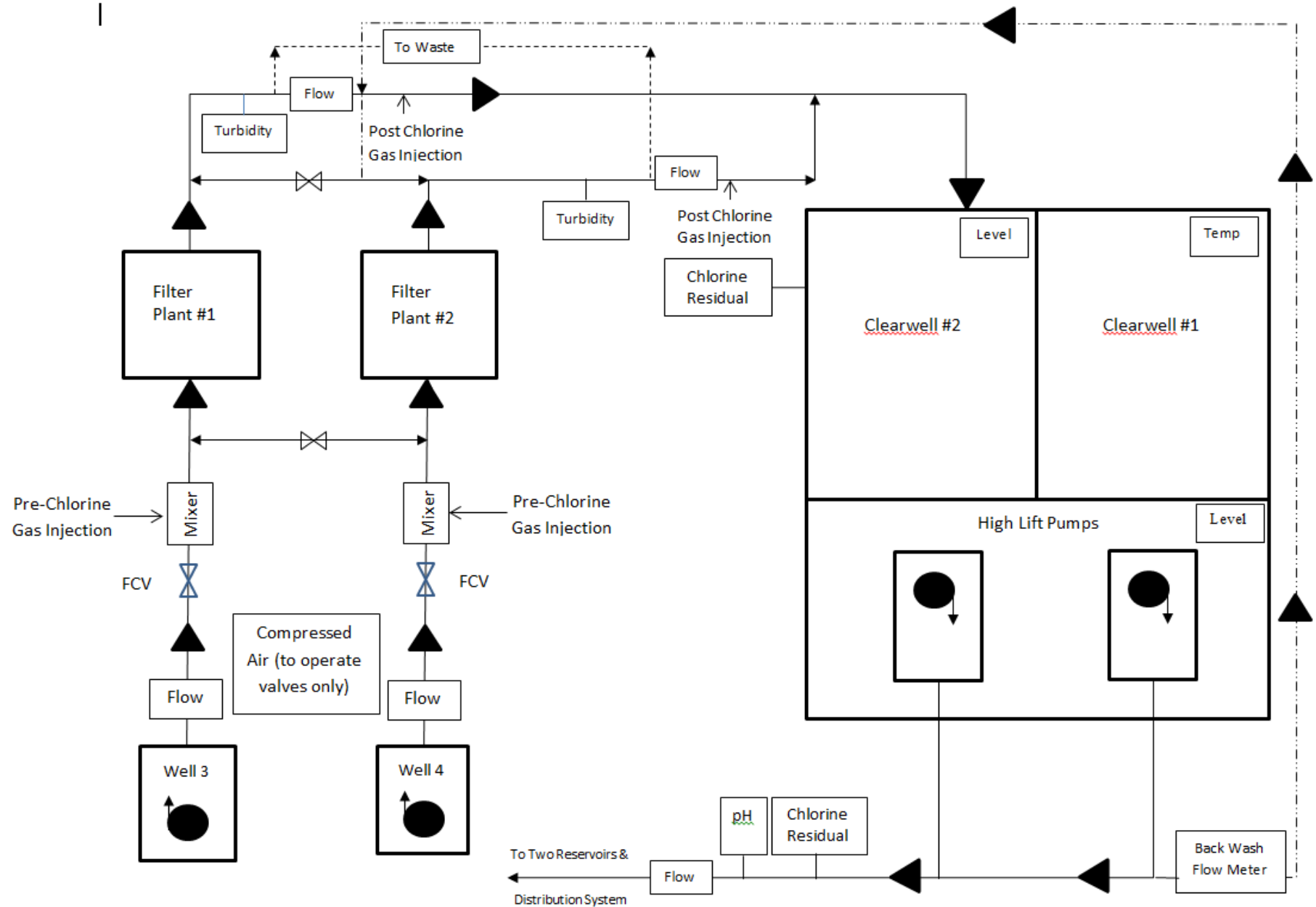
Figure 1: New Liskeard Water Treatment Plant - Process Flow & Instrumentation Diagram
