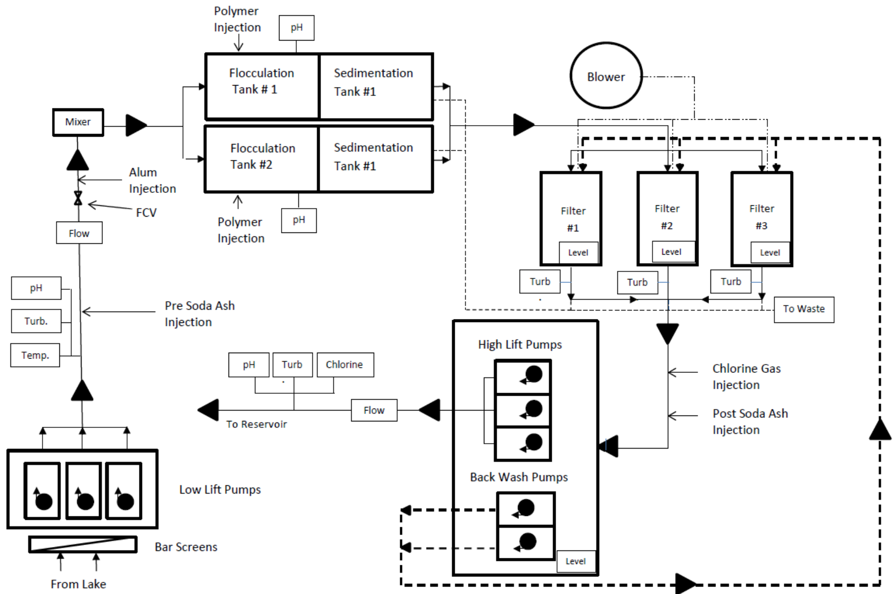
Figure 1: Haileybury Water Treatment Plant - Process Flow & Instrumentation Diagram
