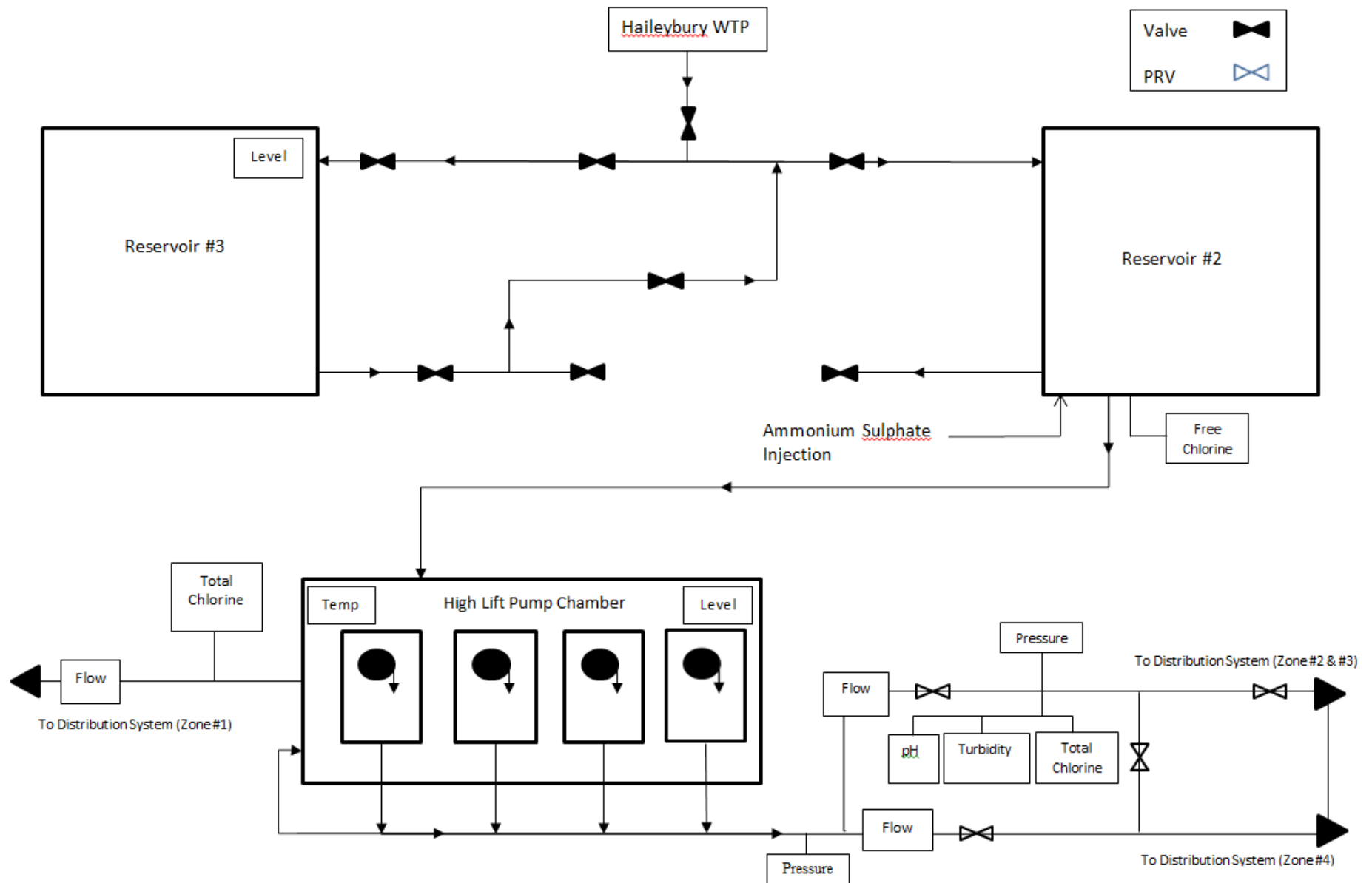
Figure 2: Haileybury Reservoir - Process Flow & Instrumentation Diagram
